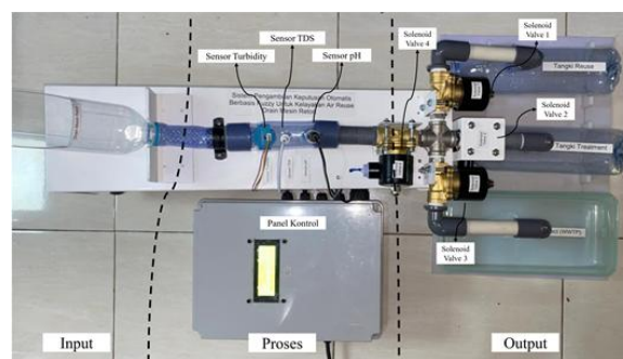
Gambar 2. Prototype Sistem
